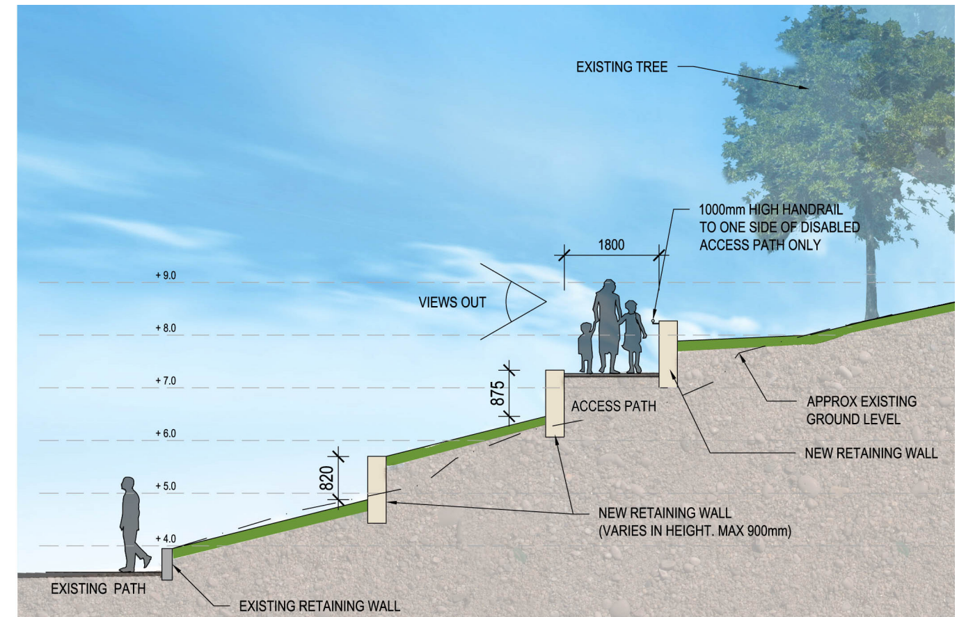
SECTION B
